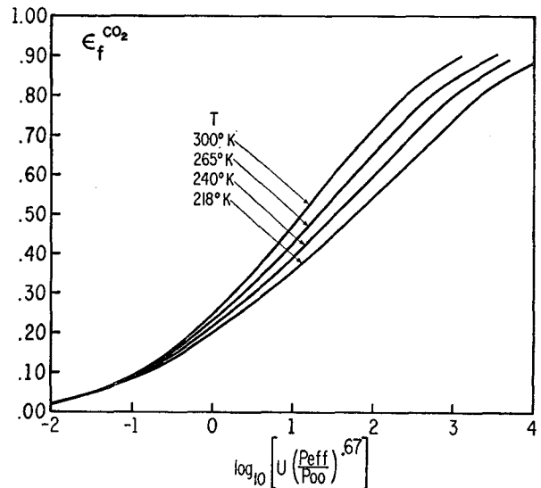
FIG. 29. Slab absorptivities of CO 2 at various temperatures.
